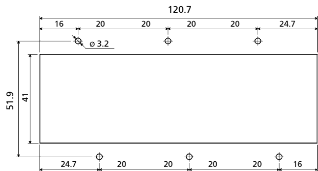
Drilling template
