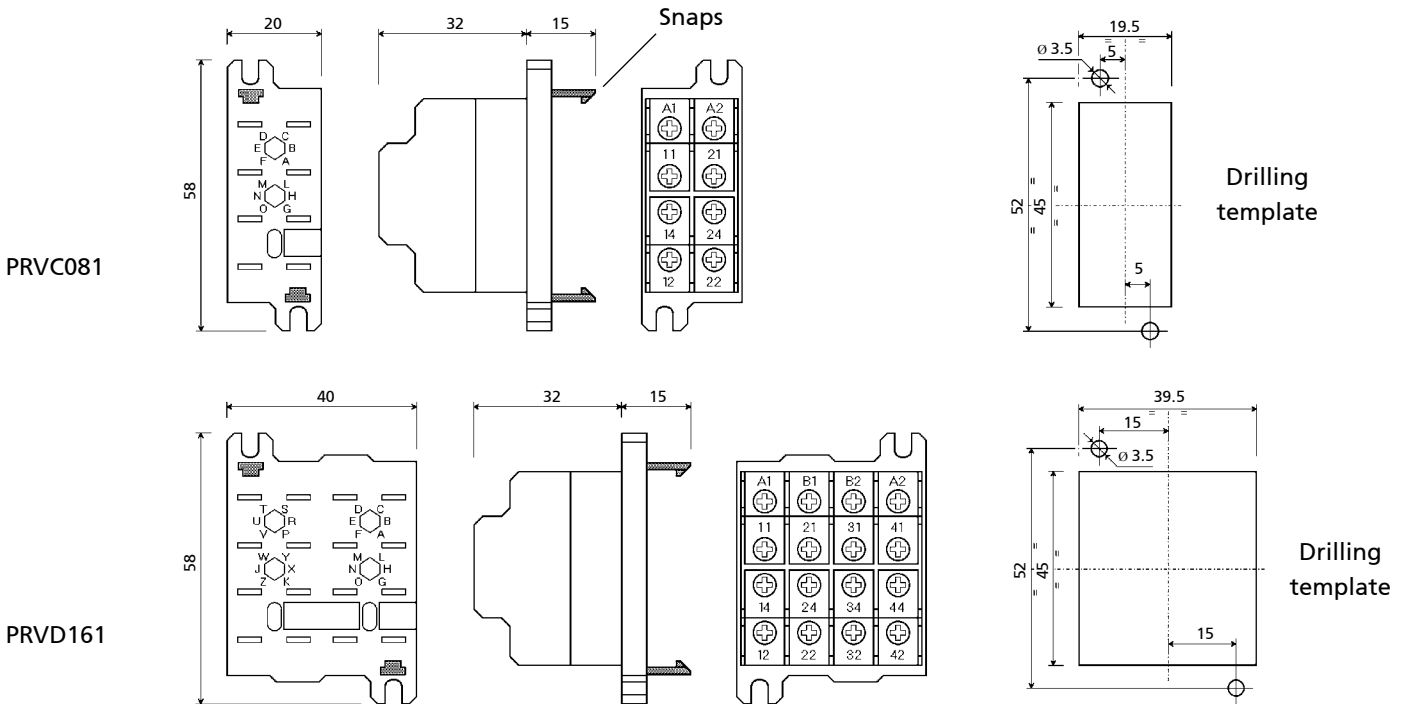
Detail of connections
