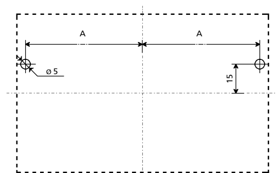
Fixing template
