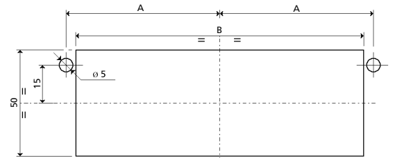
Drilling template
